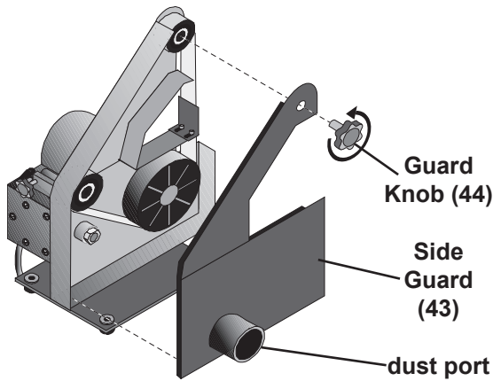
Figure A: Side Guard (43) removal
