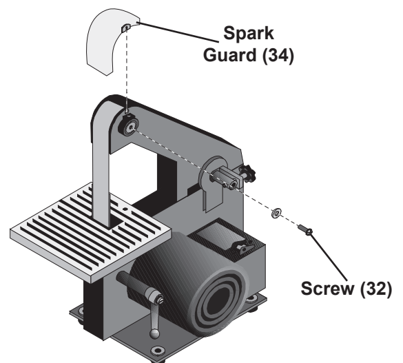
Figure C: Spark Guard (34) installation
